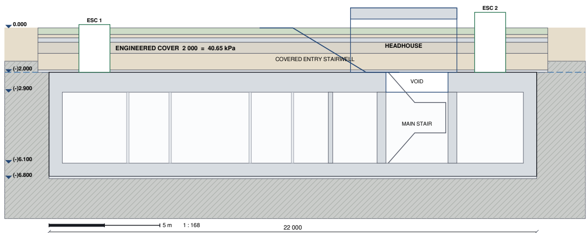
Fig 3.2 : Longitudinal Section on the Box Centreline
